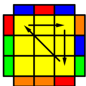
Aa type permutation
