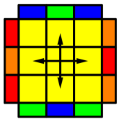
H type permutation
